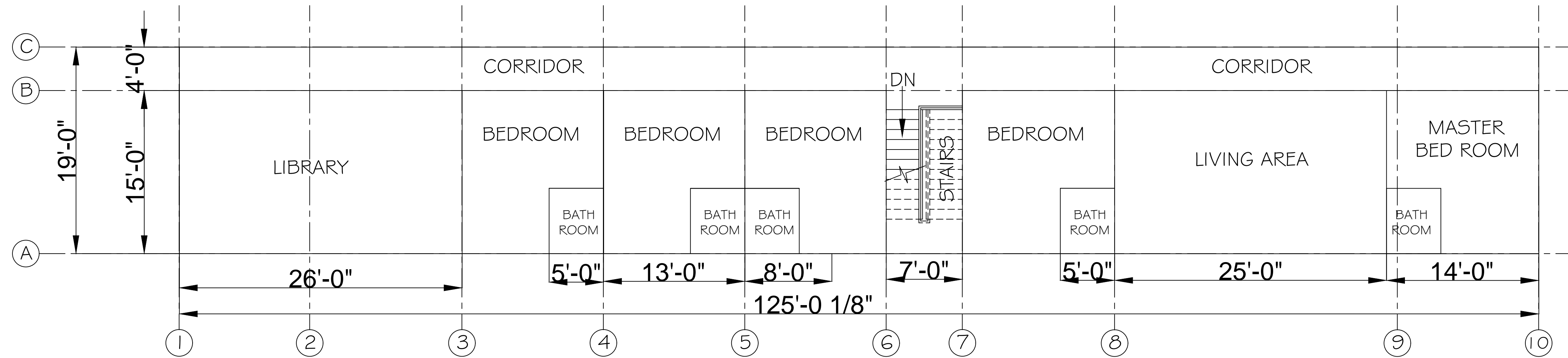
UPPER FLOOR PLAN
