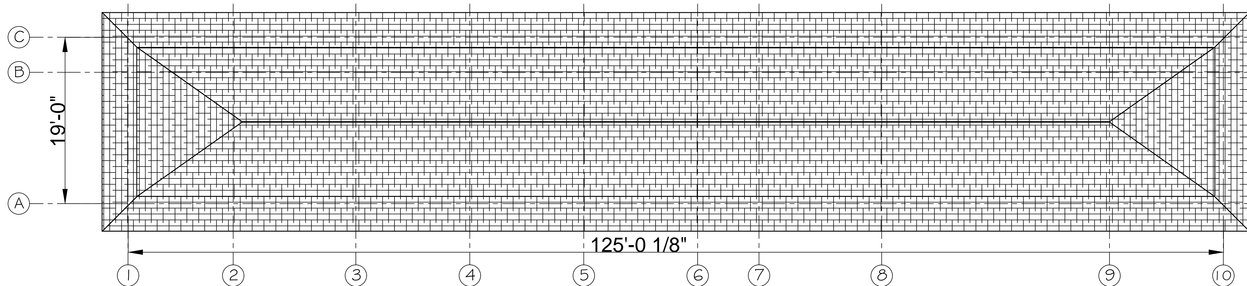
ROOF PLAN
